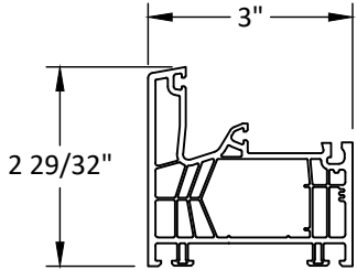
1 FRAME
