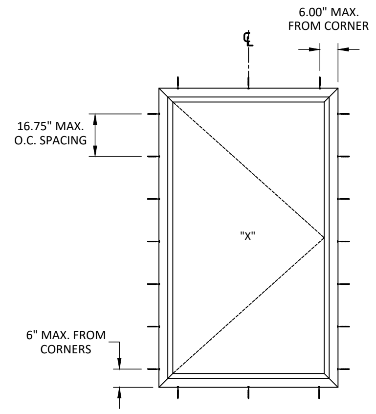
ANCHOR LAYOUT STRAP
