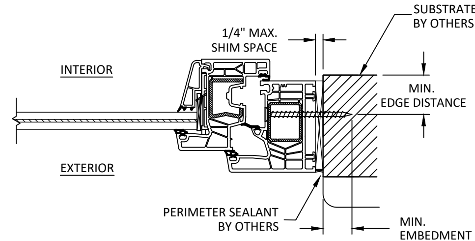
A 4 ANCHOR DETAIL THROUGH FRAME (JAMB)
