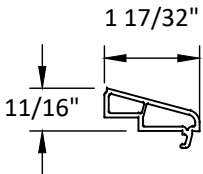
5 LAMI GLAZING BEAD
