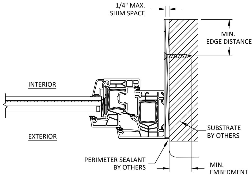
B 4 ANCHOR DETAIL STRAP (JAMB)
